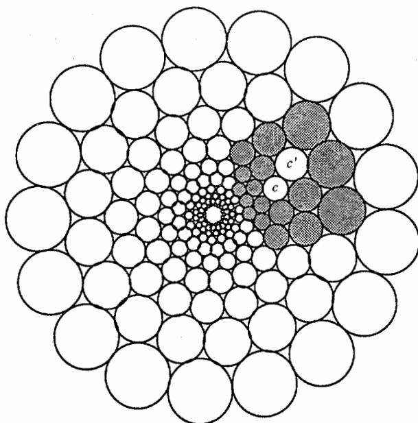
FIGURE 4.3. Two generations: 1 - s_2 < (\text{radius } c_1)/(\text{radius } c_2) < 1 + s_2
